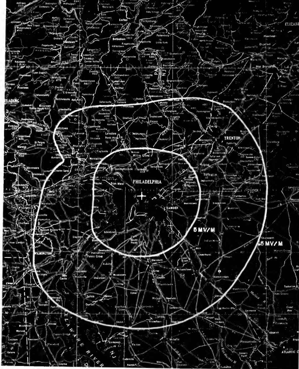
Contour map shows primary area with calculated signal strength of 5 millivolts and secondary area with calculated 0.5 millivolt signal limit.
